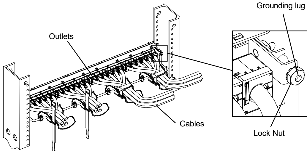
24-Port Panel Ground
