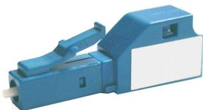
Fiber Optic Power Reducing Build Out Attenuator, singlemode LC/UPC, 1dB, blue
